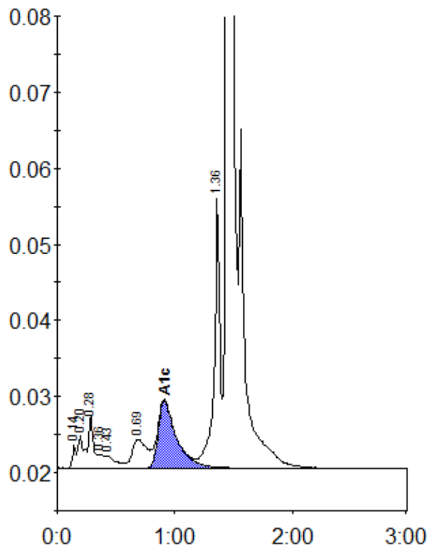
Peak table - ID: 10597035
